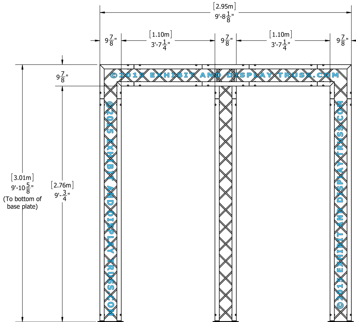
Front View Units: Feet & Inches Metres
