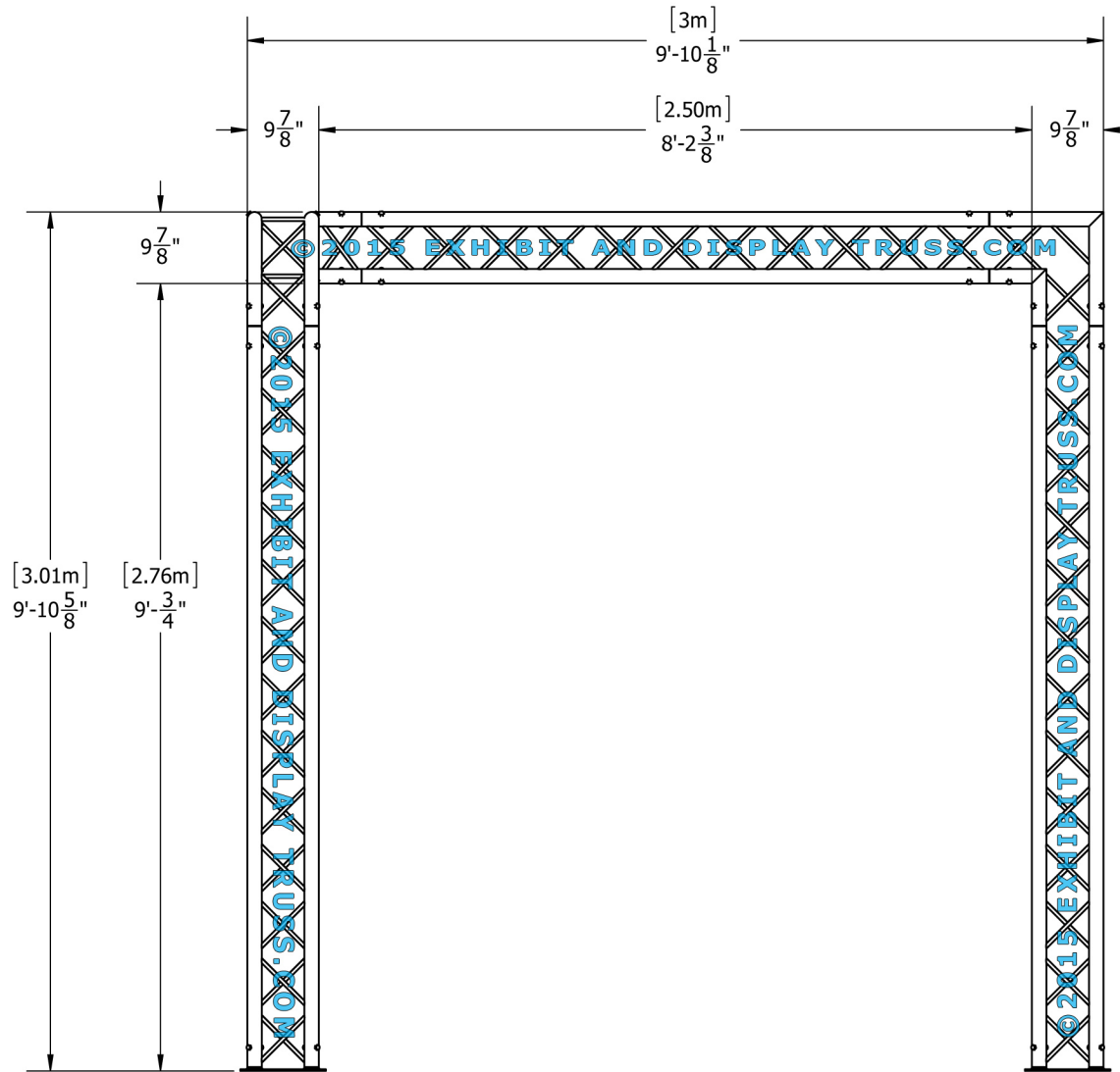
SIDE VIEW UNITS: FEET & INCHES METRES
