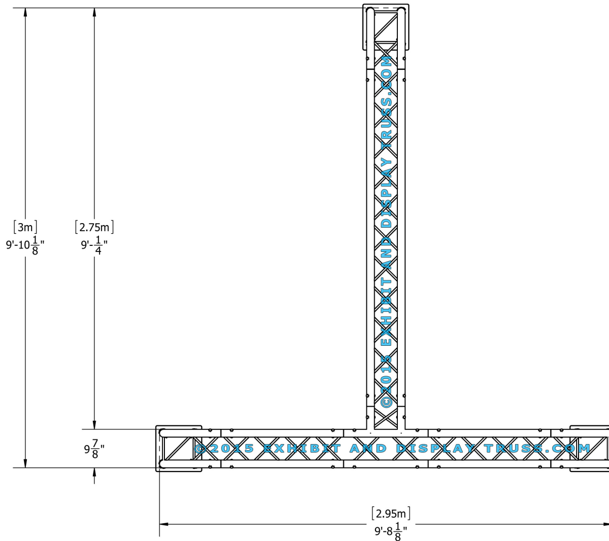
Top View Units: Feet & Inches Metres
