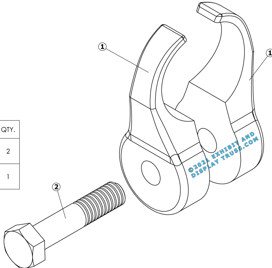
EXPLODED VIEW
