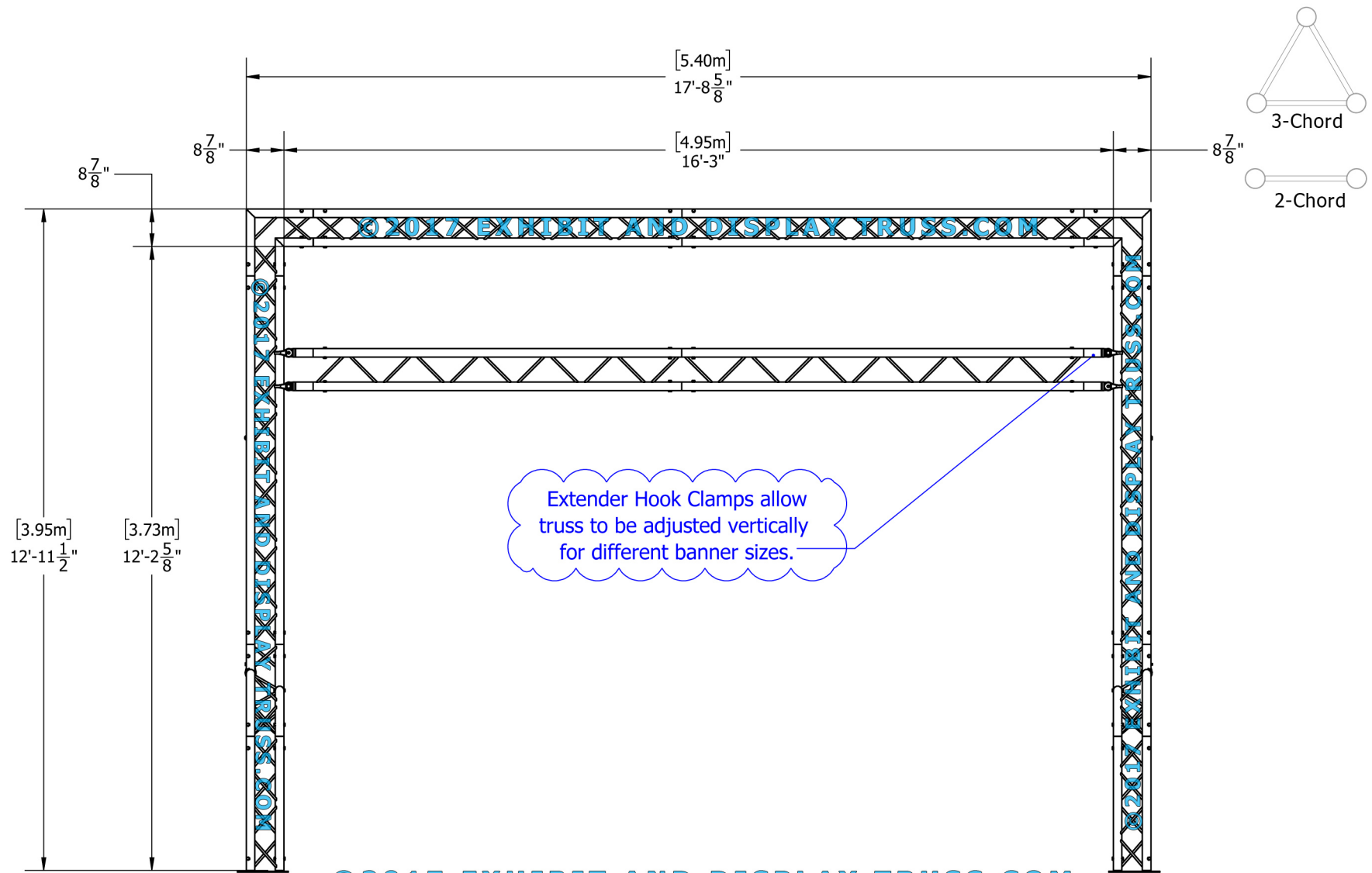
Front View Units: Feet & Inches [Meters]
